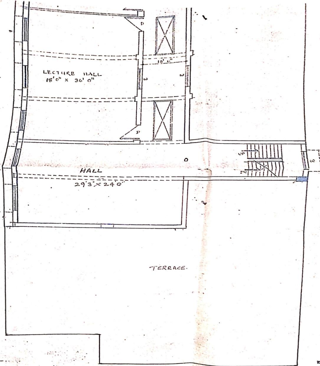
PROPOSED SECOND FLOOR PLAN - BLOCK - A
