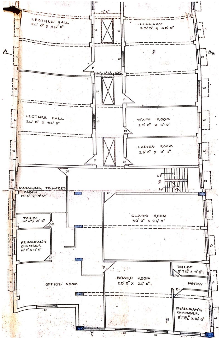
EXISTING FIRST FLOOR PLAN - BLOCK-A
